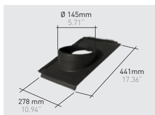
Q87*K | Planum chimney roof tile klinker
