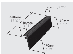
Q88*K | Planum right side course / Rake klinker
