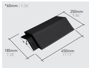
Q90*K | Atica ridge 120° klinker
